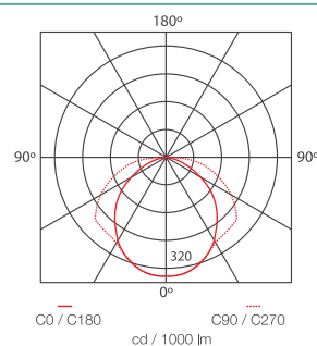
Veil LIT 3000 lm 2X2 opal
