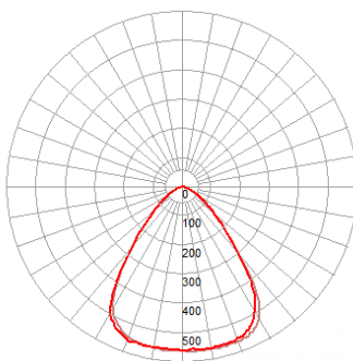
High Bay GC015 100W
