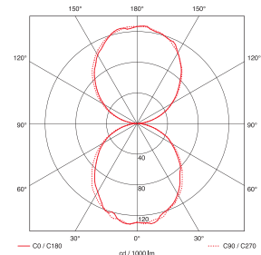
UL ARIA LED SMD-S2 2 2600 lm 24 AB-AR
