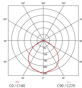
cd / 1000 lm ARIA FL 24" x 24" 90° 3000Lm
